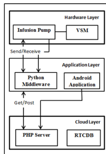
Figure 4. Three Layer Architectural Model for Patient Monitoring
